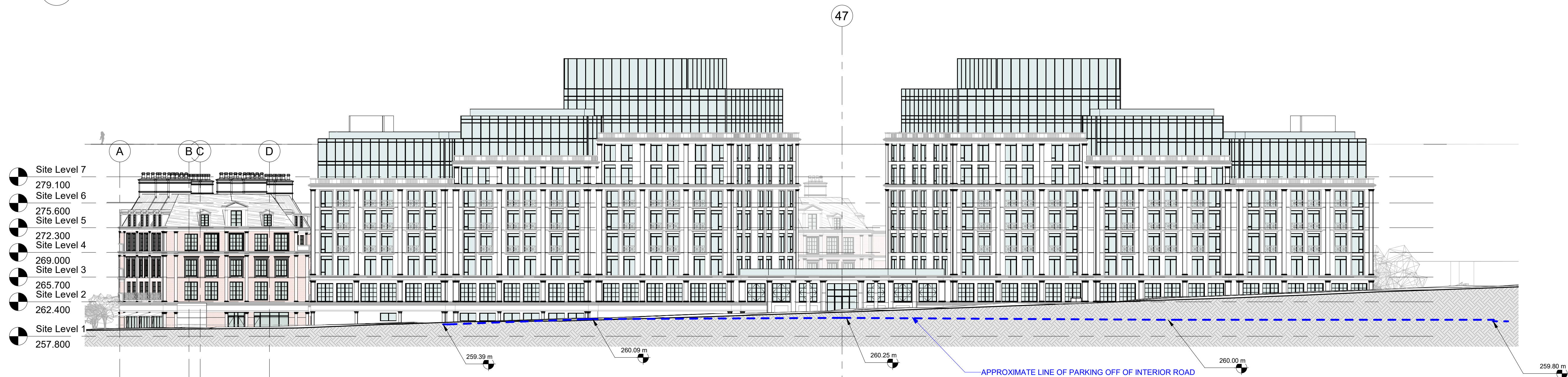
3 Site Section-03 Through Yonge Street A-301 1 : 300
