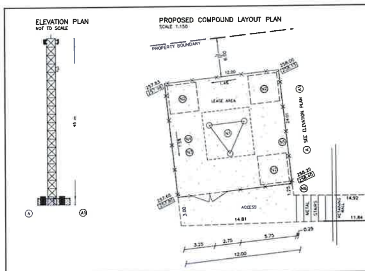
Figure 1: Compound Layout
